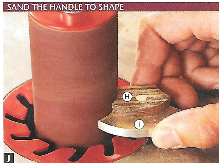
J Sand the sides of the handle assembly (H/I) on progressively finer sanding drums to achieve the sheen you desire on the metal.
