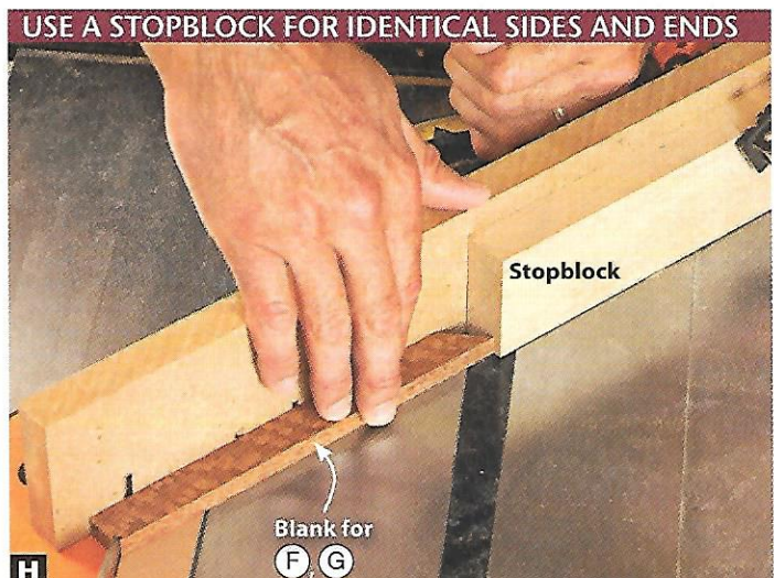
H Position the miter-gauge head as shown so the workpiece presses against the stopblock throughout the cut.
