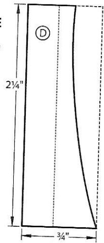
FOOT FULL-SIZE PATTERN SIDE VIEW
