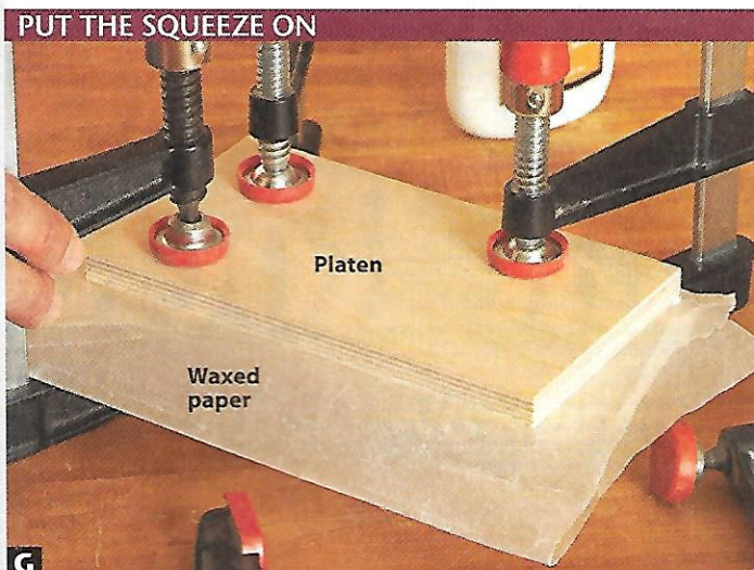
G After gluing veneer on both faces, place waxed paper on top of the veneered panel, then clamp the top platen in place.
