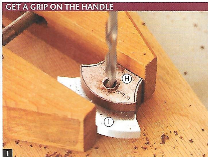
I Clamp the handle base (H) and handle (I) in a handscrew. Mount a 1/4" twist bit in your drill press and bore through both pieces.
