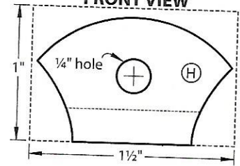
HANDLE BASE FULL-SIZE PATTERN FRONT VIEW
